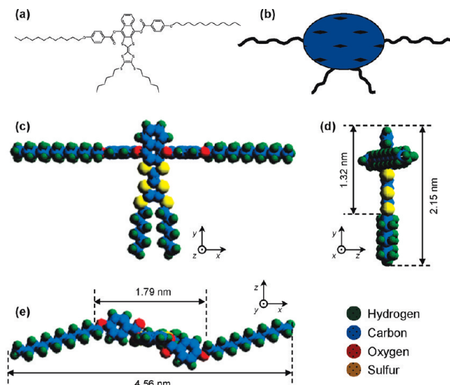
Figure 1. Chemical structure (a) and schematic illustration (b) of investigated a-6TTF12 molecule. Calculated geometric dimensions of a-6TTF12 molecule in the views from the z -axis (c), x -axis (d), and y -axis (e), respectively.
